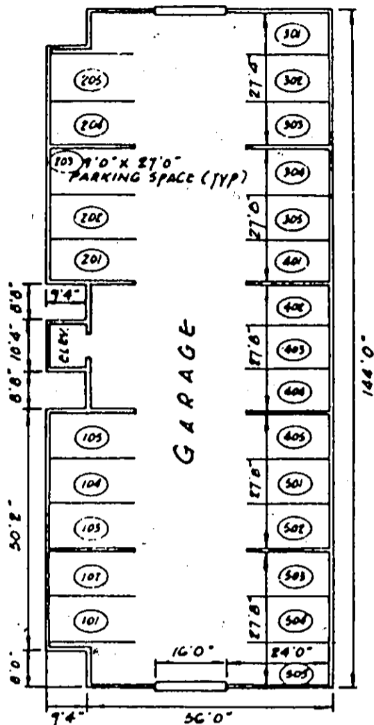
GARAGE FLOOR PLAN
