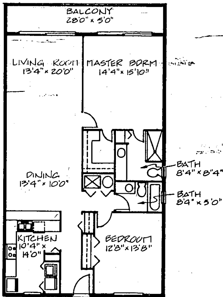
TYPICAL LIVING AREA
